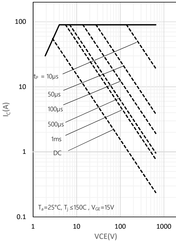
Fig. 1 FBSOA characteristics
