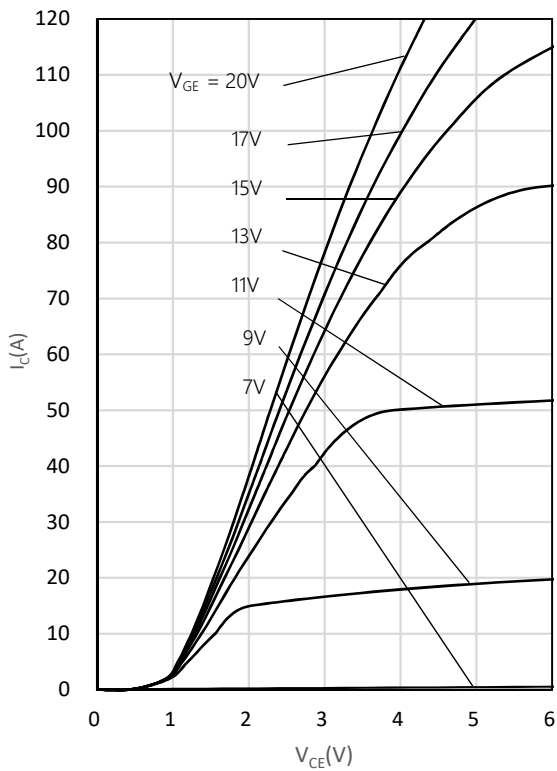
Fig. 3 Output characteristics
