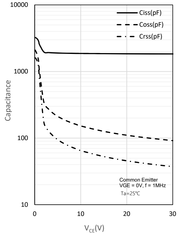
Fig. 10 Capacitance characteristics
