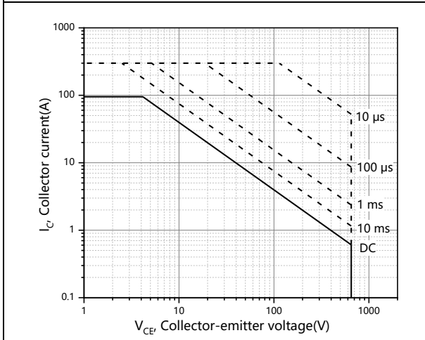
Figure 9. Safe operation area T_C=25^{\circ}C
