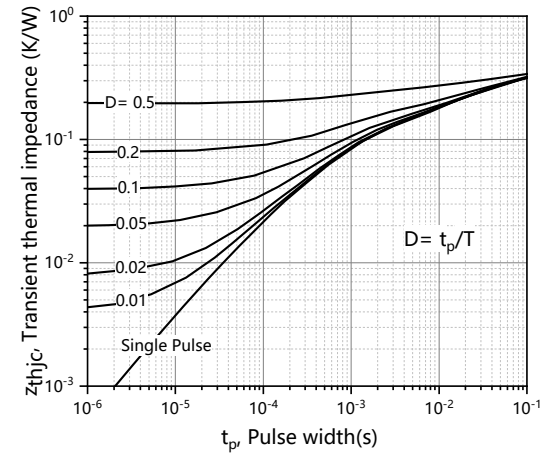
Figure 10. IGBT transient thermal impedance
