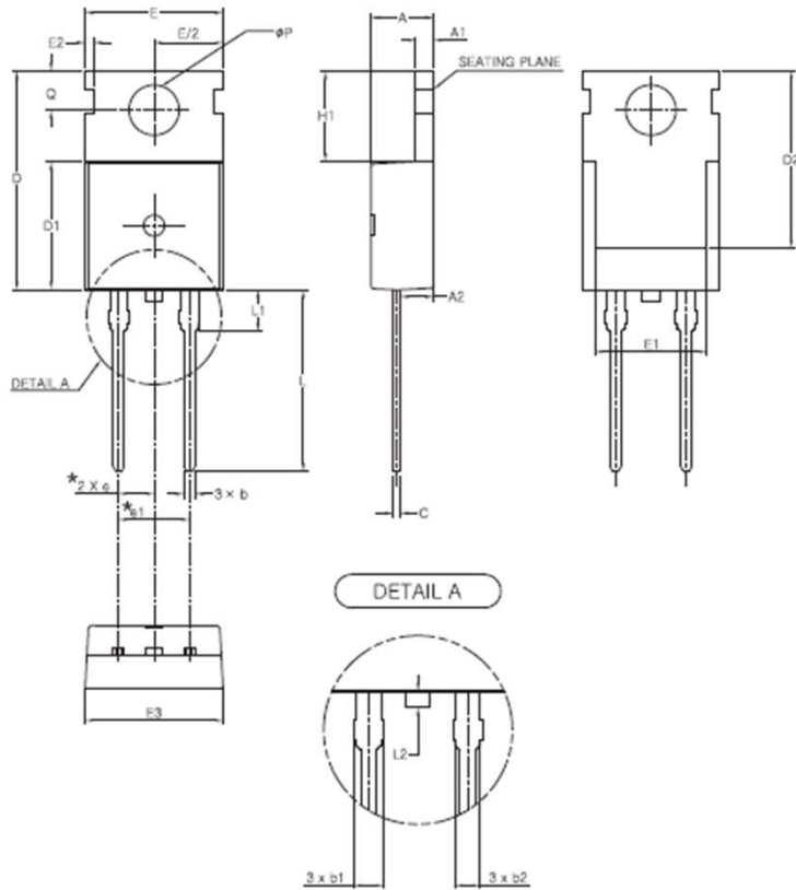
TO-220-2L
