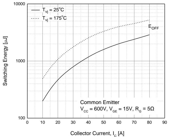
Fig. 12 Turn-off Loss vs. Collector Current
