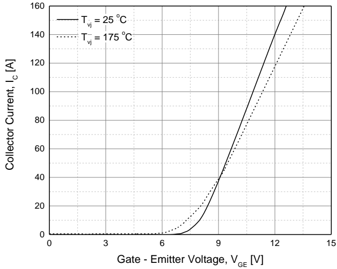
Fig. 5 IGBT Transfer Characteristic
