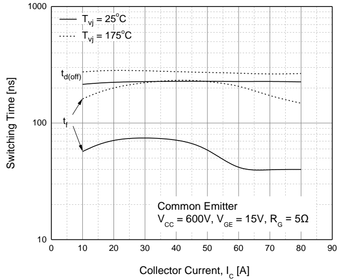
Fig. 10 Turn-off Time vs. Collector Current
