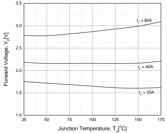
Fig. 8 Diode Forward Voltage vs. Junction Temperature
