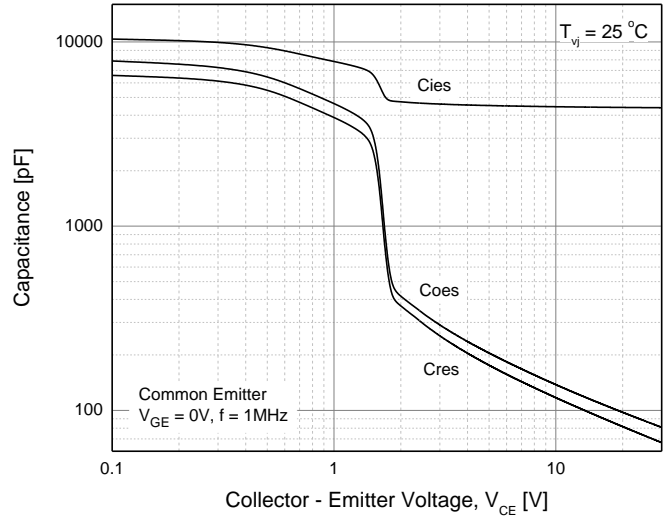
Fig. 6 IGBT Capacitance Characteristics
