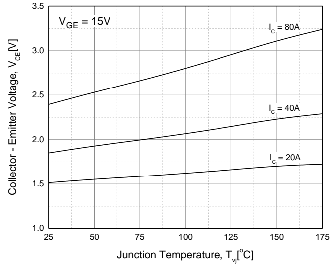
Fig. 3 IGBT Saturation Voltage vs. Junction Temperature
